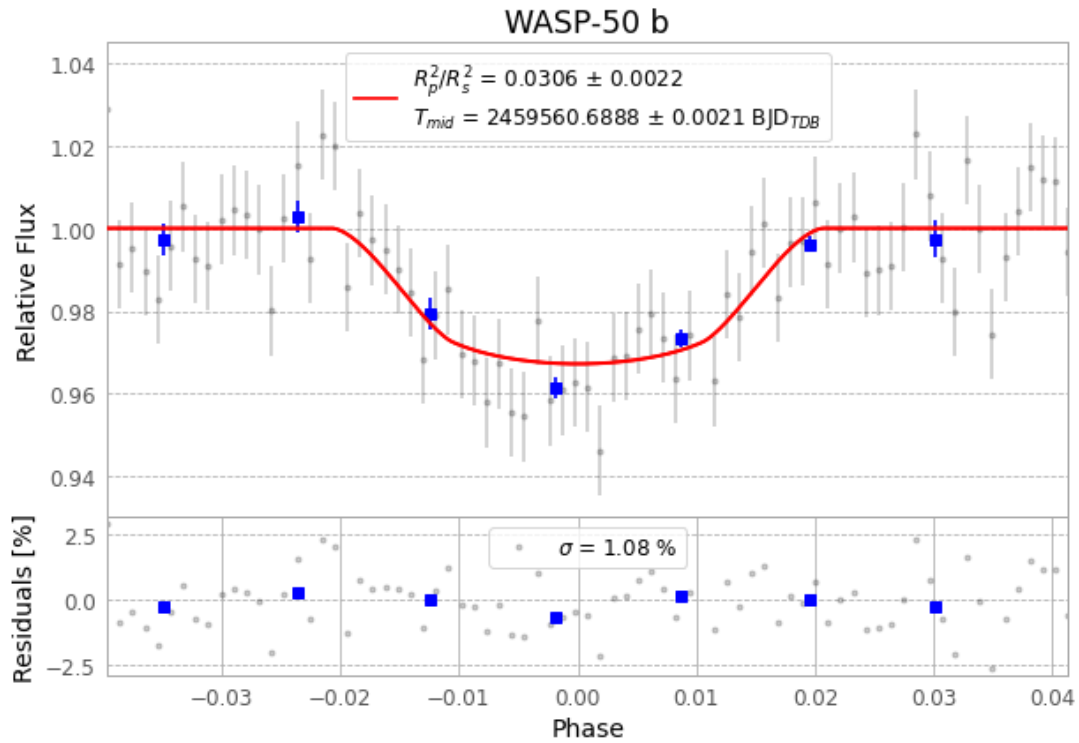
Figure 1 — FinalLightCurve_WASP-50 b_2021-12-11.png (SHA-256 c08cd7f5f98b06aa...)
