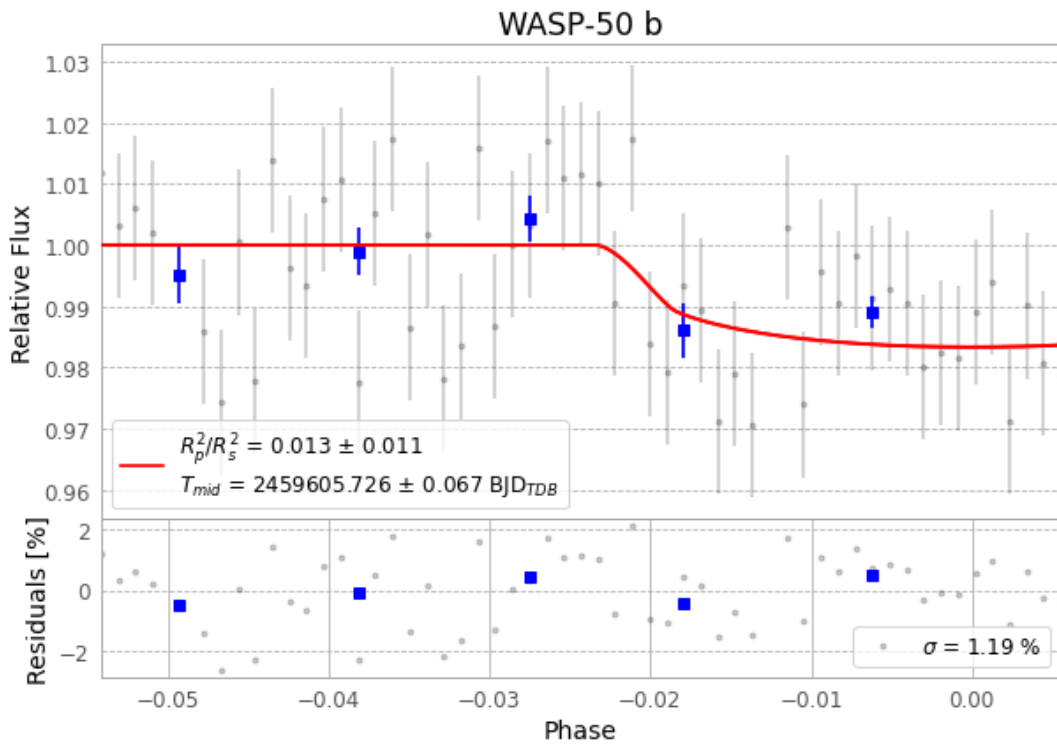
Figure 1 — FinalLightCurve_WASP-50 b_2022-01-25.png (SHA-256 5c3a4467870940f6...)
