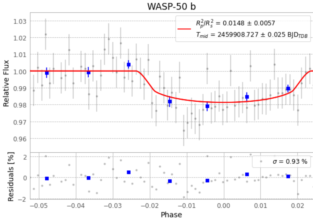
Figure 1 — FinalLightCurve_WASP-50 b_2022-11-24.png (SHA-256 6776ce974d422daf...)
