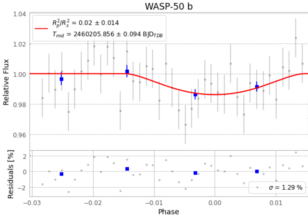
Figure 1 — FinalLightCurve_WASP-50 b_2023-09-17.png (SHA-256 d8f6c72cac9d1825...)
