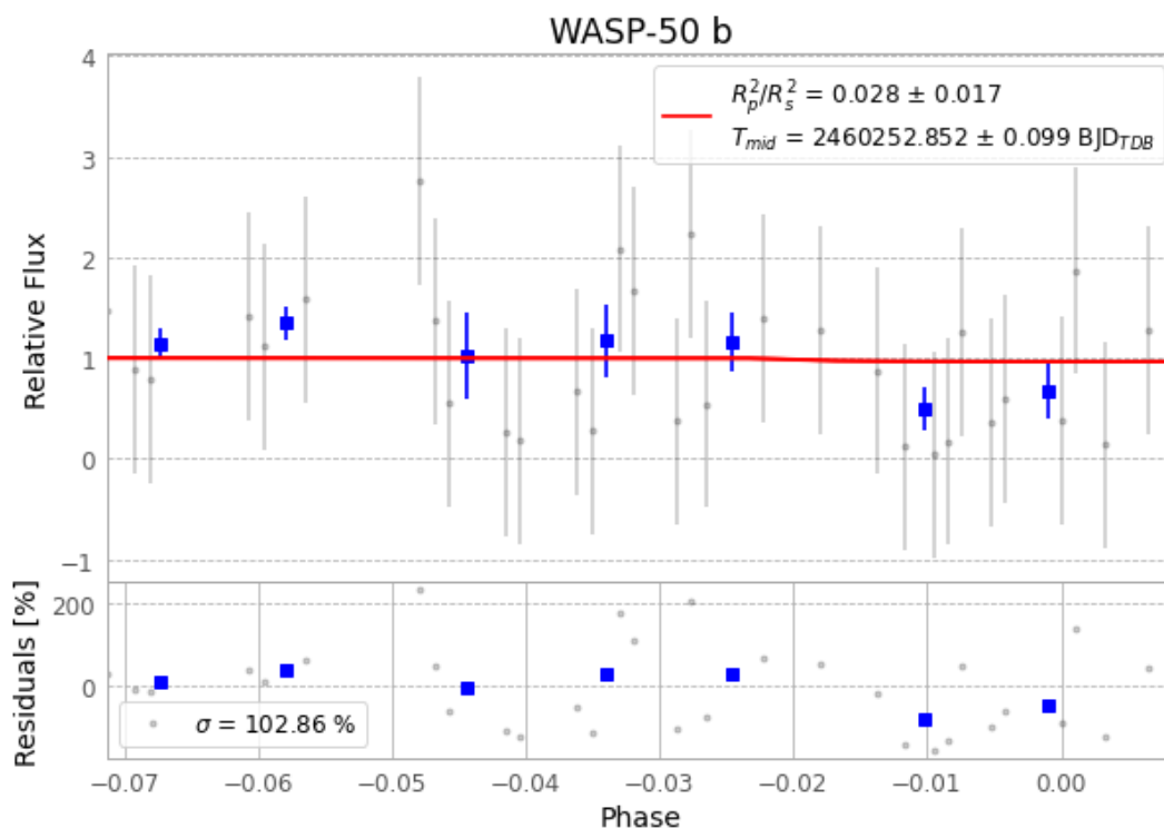
Figure 1 — FinalLightCurve_WASP-50 b_2023-11-03.png (SHA-256 ce483c80caf7f61f...)
