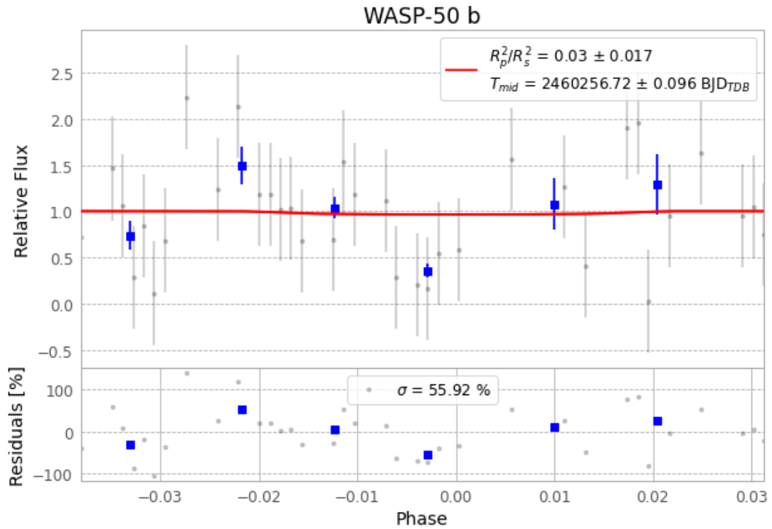
Figure 1 — FinalLightCurve_WASP-50 b_2023-11-07.png (SHA-256 9d25719d8a5dd35c...)
