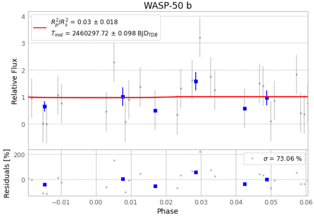
Figure 1 — FinalLightCurve_WASP-50 b_2023-12-18.png (SHA-256 5a8b9ed38ce0a23f...)
