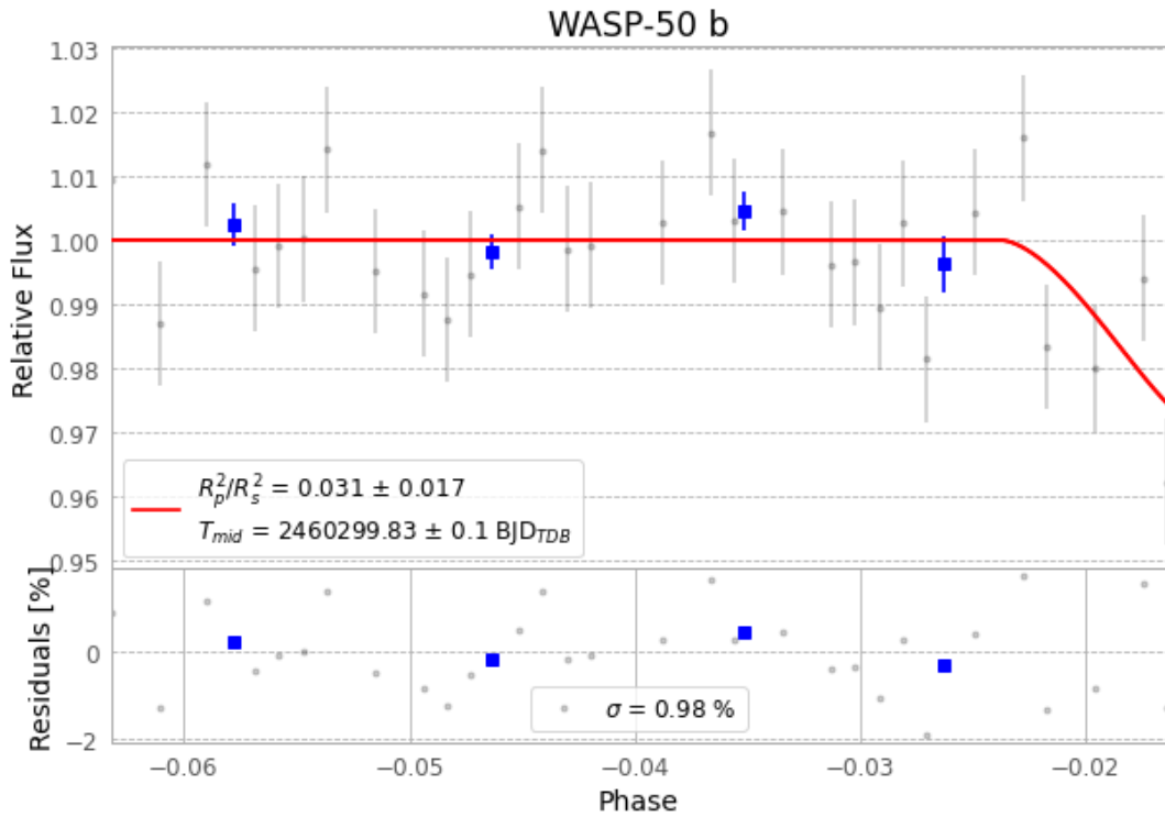
Figure 1 — FinalLightCurve_WASP-50 b_2023-12-20.png (SHA-256 3e21a0ec9526938a...)
