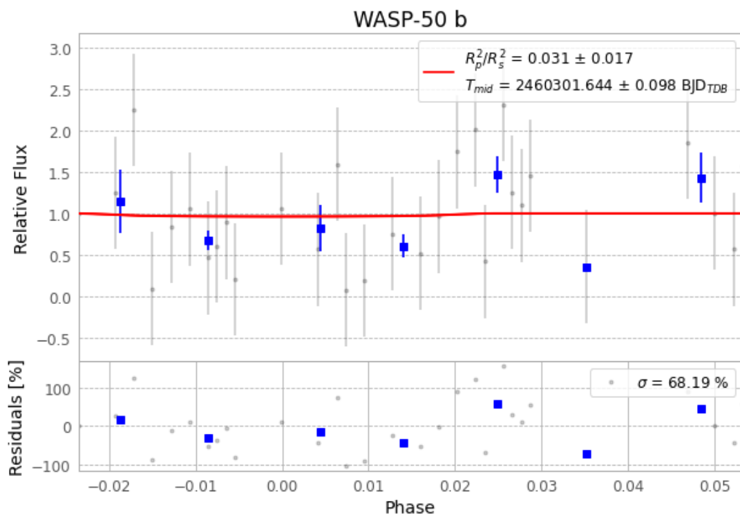
Figure 1 — FinalLightCurve_WASP-50 b_2023-12-22.png (SHA-256 438e399845bf946e...)
