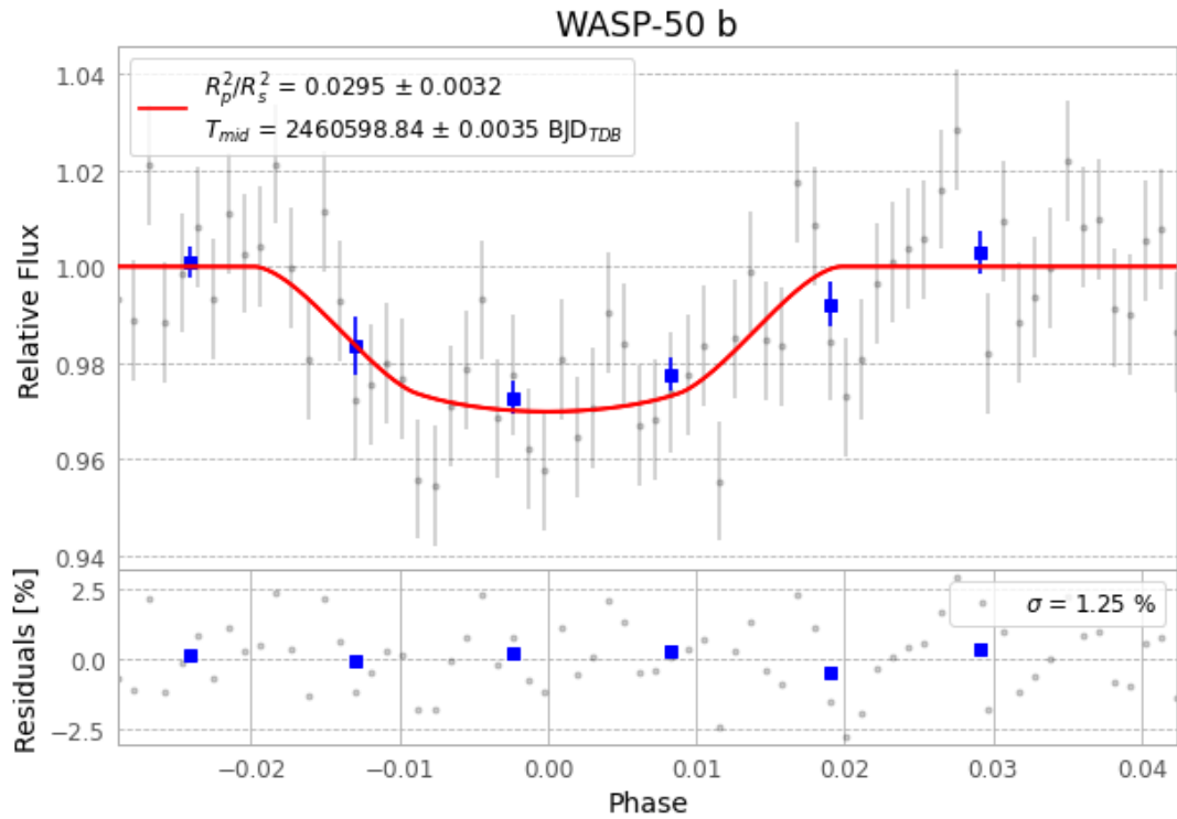
Figure 1 — FinalLightCurve_WASP-50 b_2024-10-14.png (SHA-256 a5c1714371d825f6...)
