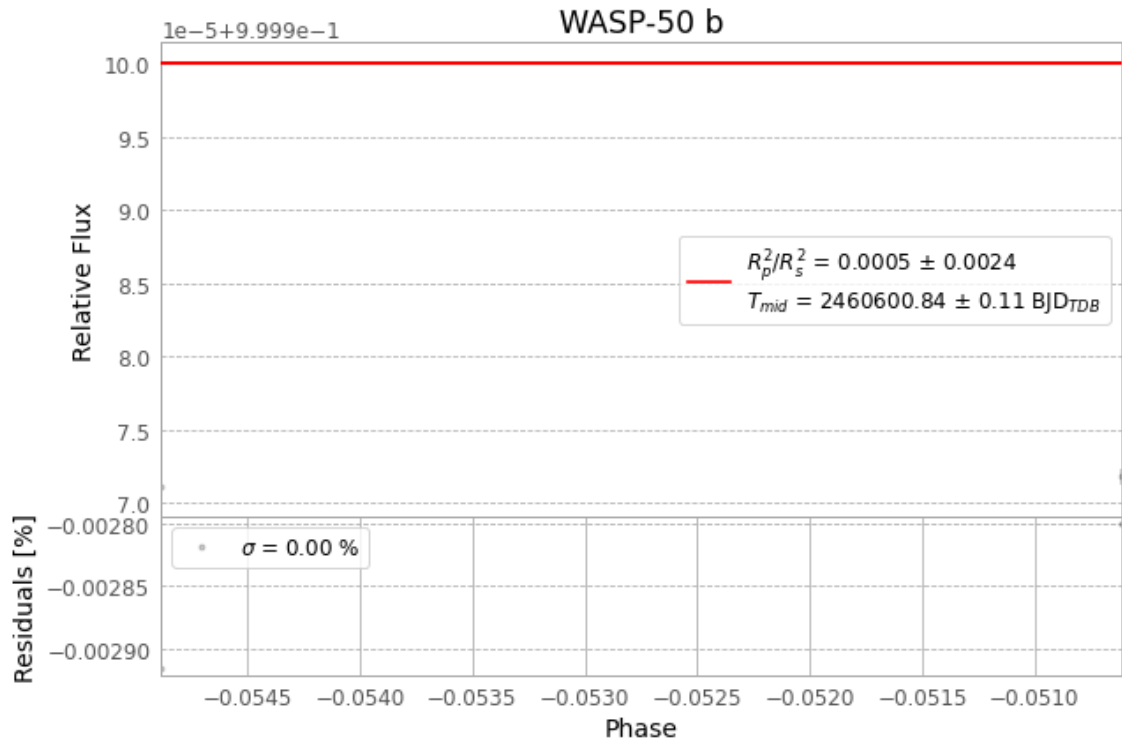
Figure 1 — FinalLightCurve_WASP-50 b_2024-10-18.png (SHA-256 91abfc706abb0469...)
