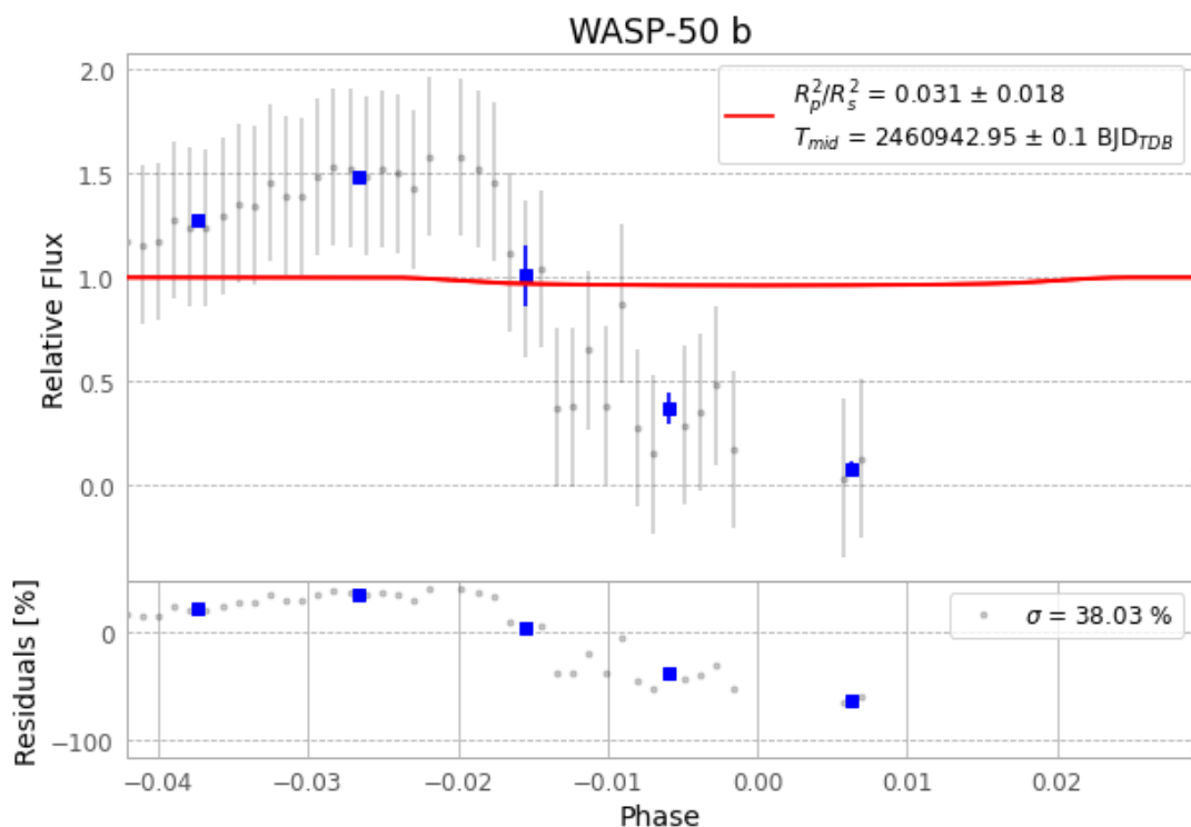
Figure 1 — FinalLightCurve_WASP-50 b_2025-09-24.png (SHA-256 80200e81b8e60835...)
