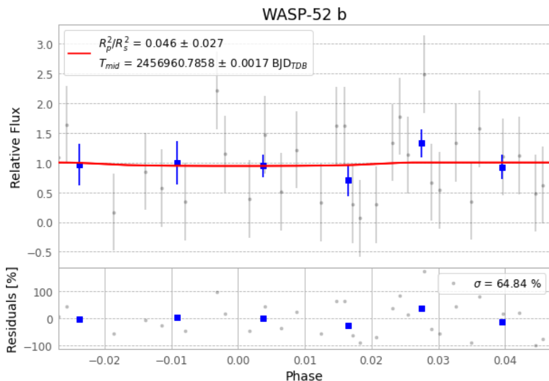
Figure 1 — FinalLightCurve_WASP-52 b_2014-10-29.png (SHA-256 9a5f5f39526d5d23...)
