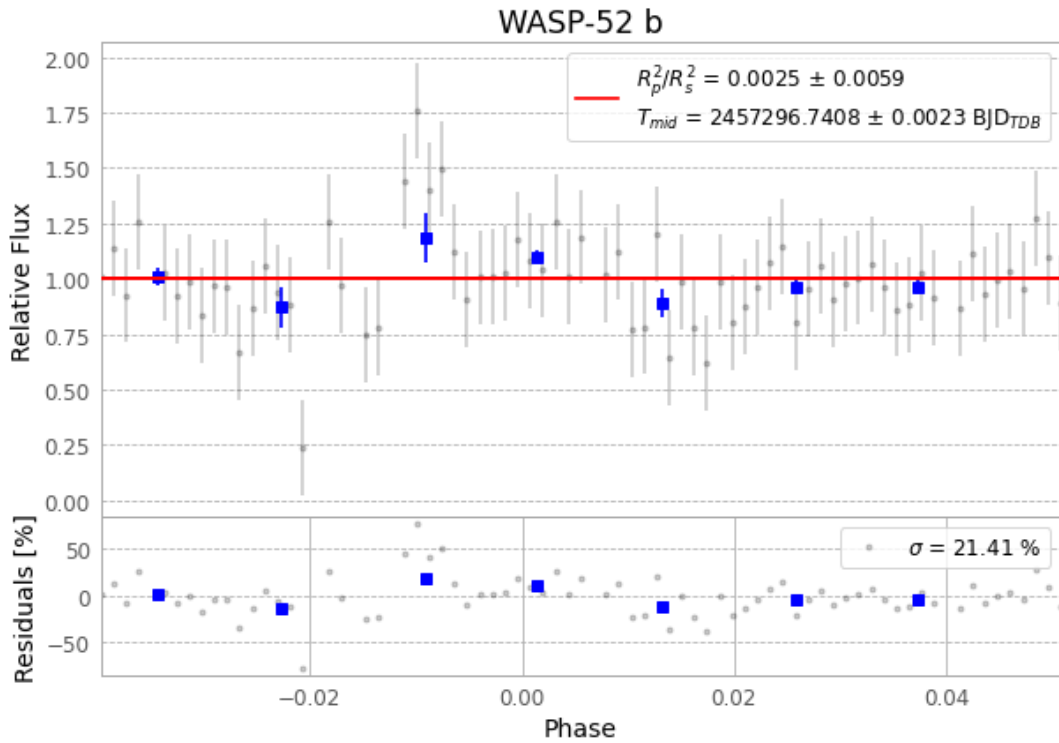
Figure 1 — FinalLightCurve_WASP-52 b_2015-09-30.png (SHA-256 18dc4a0f4b82baee...)
