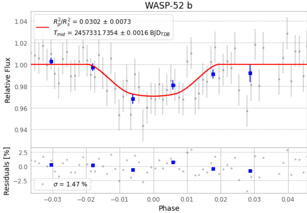
Figure 1 — FinalLightCurve_WASP-52 b_2015-11-04.png (SHA-256 123c6113635f4793...)
