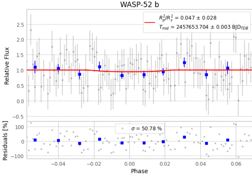
Figure 1 — FinalLightCurve_WASP-52 b_2016-09-21.png (SHA-256 f50507f3d607058a...)
