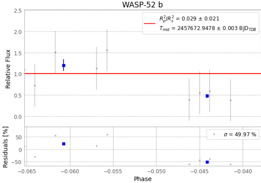
Figure 1 — FinalLightCurve_WASP-52 b_2016-10-12.png (SHA-256 029364394a168c01...)
