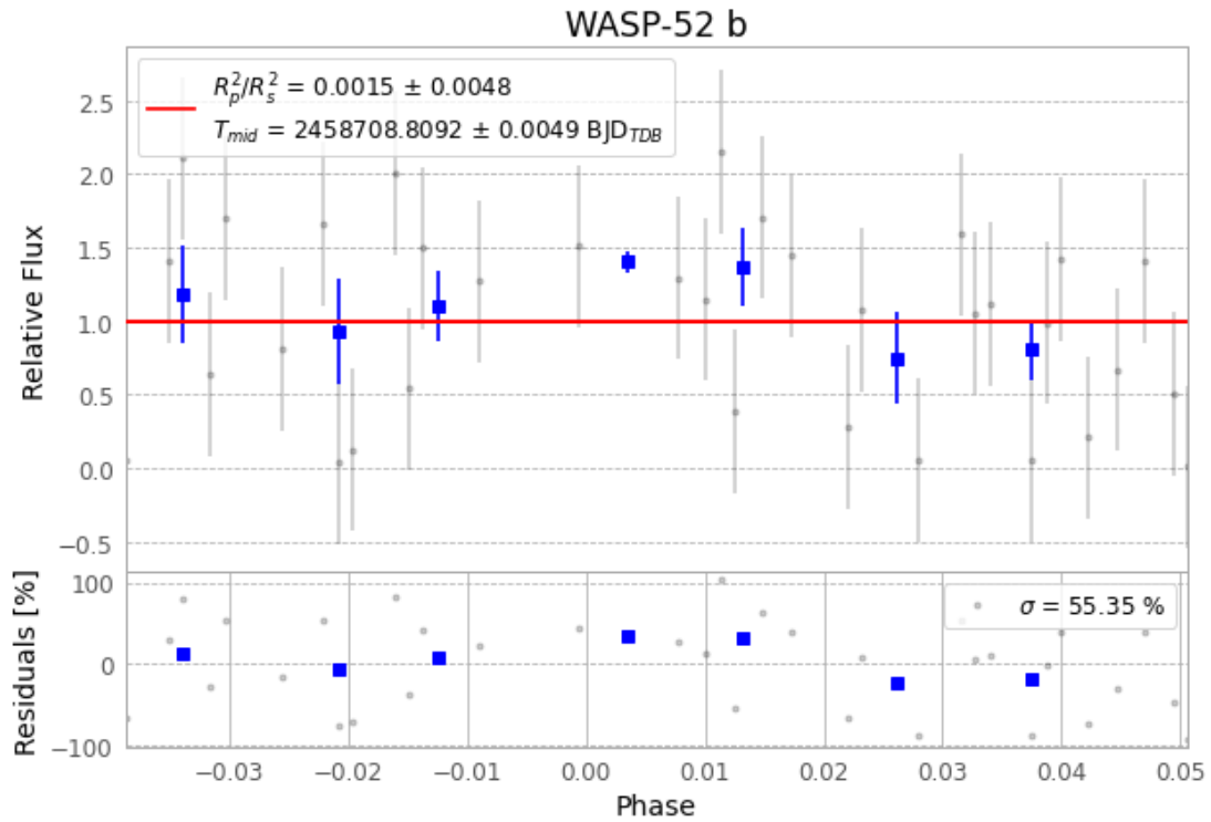
Figure 1 — FinalLightCurve_WASP-52 b_2019-08-12.png (SHA-256 1d63471500c0689e...)
