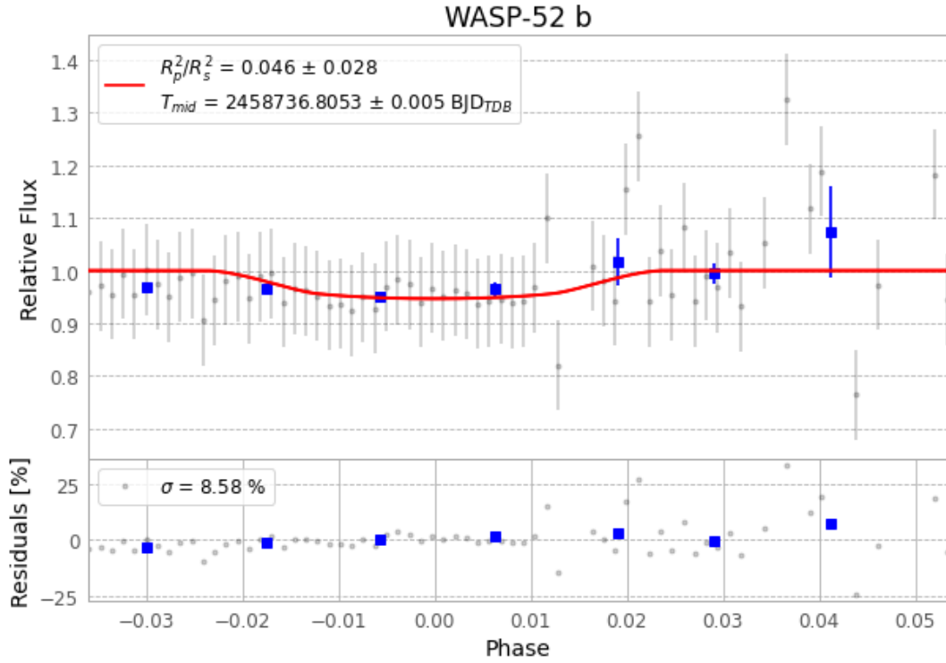
Figure 1 — FinalLightCurve_WASP-52 b_2019-09-09.png (SHA-256 4e6203522806aa91...)
