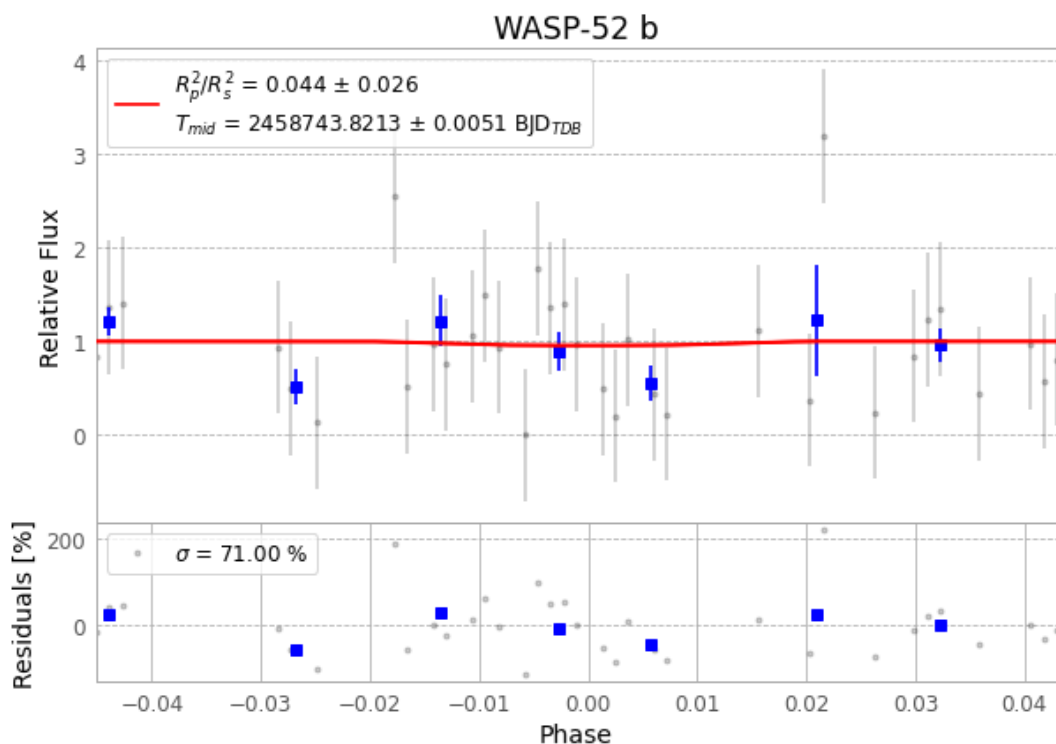
Figure 1 — FinalLightCurve_WASP-52 b_2019-09-16.png (SHA-256 83d93692bc8a6627...)
