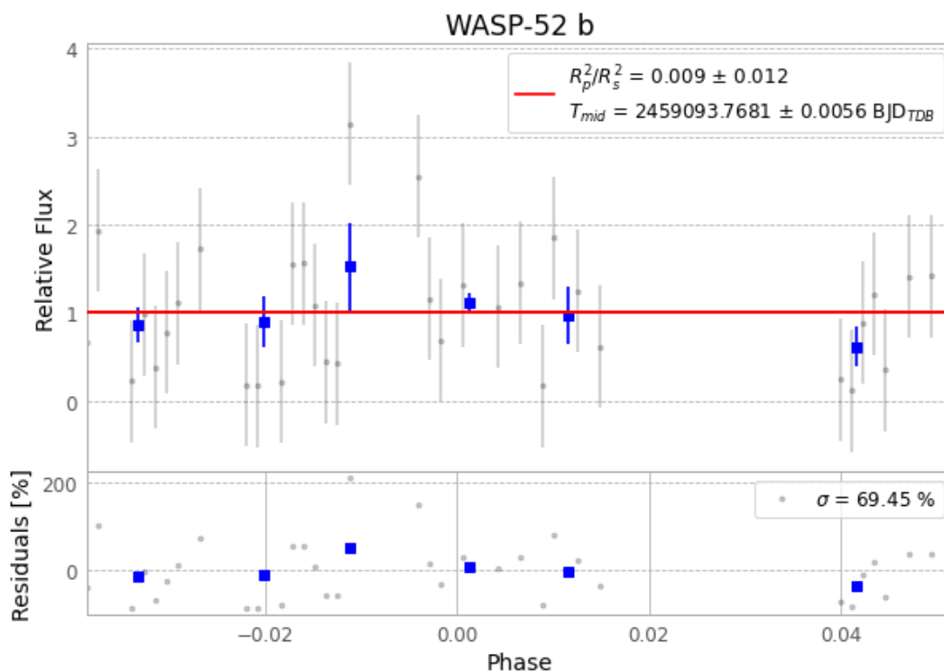
Figure 1 — FinalLightCurve_WASP-52 b_2020-08-31.png (SHA-256 7831c466bbce9861...)
