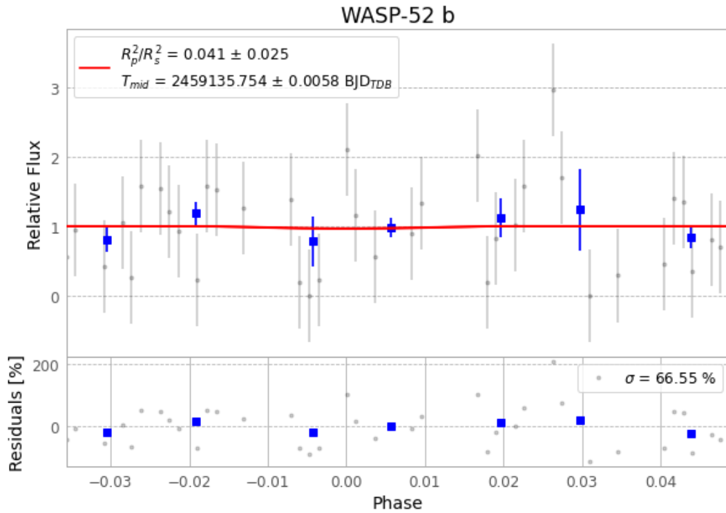
Figure 1 — FinalLightCurve_WASP-52 b_2020-10-12.png (SHA-256 98a45858f0875f64...)
