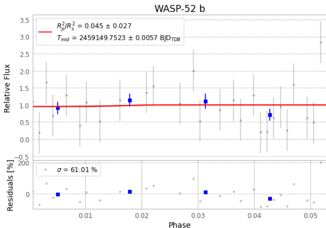
Figure 1 — FinalLightCurve_WASP-52 b_2020-10-26.png (SHA-256 6a7b2ab8a9492d01...)
