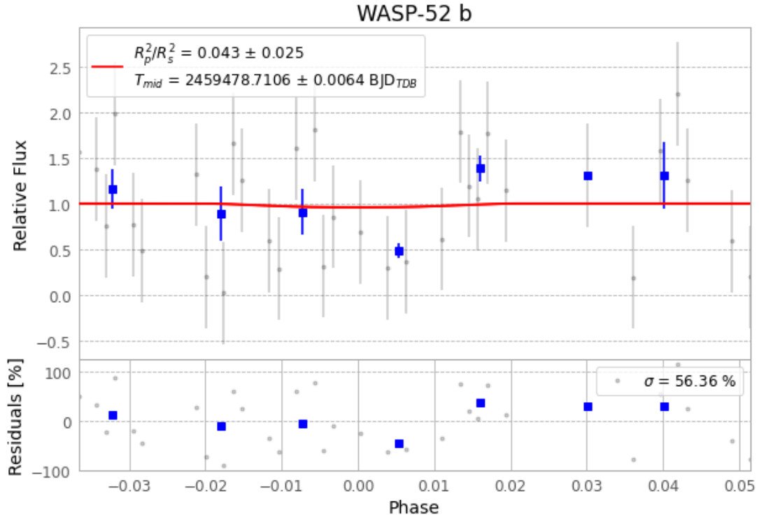
Figure 1 — FinalLightCurve_WASP-52 b_2021-09-20.png (SHA-256 3d801068f6197504...)
