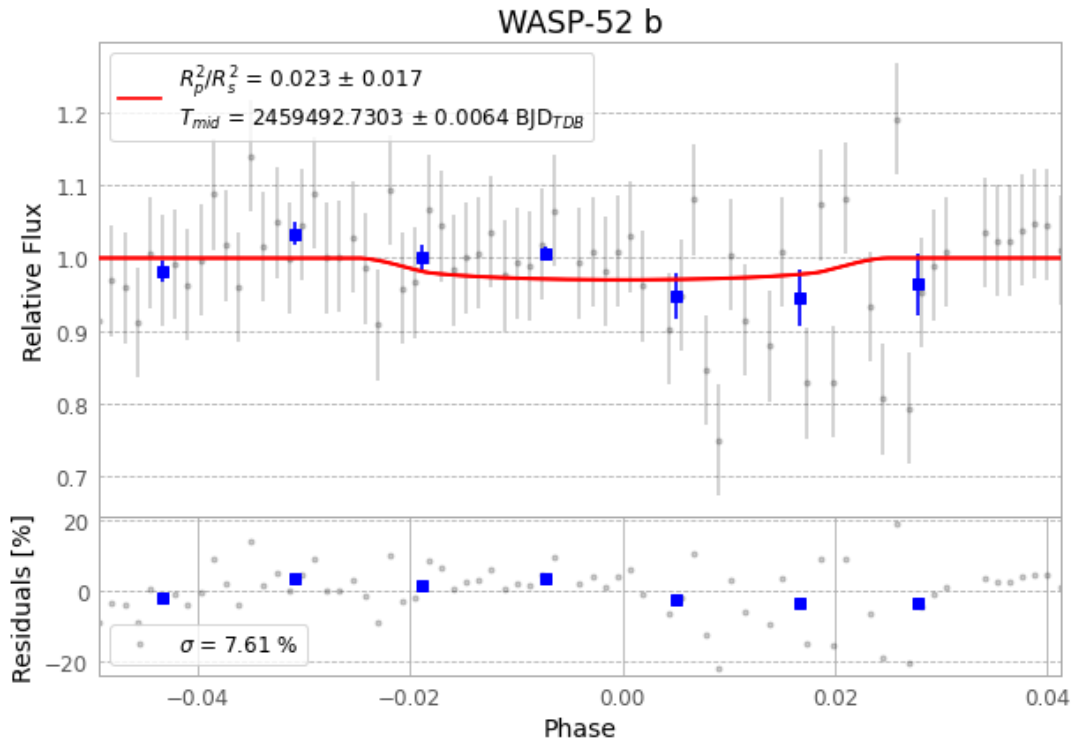
Figure 1 — FinalLightCurve_WASP-52 b_2021-10-04.png (SHA-256 407b9cbcd8546e54...)
