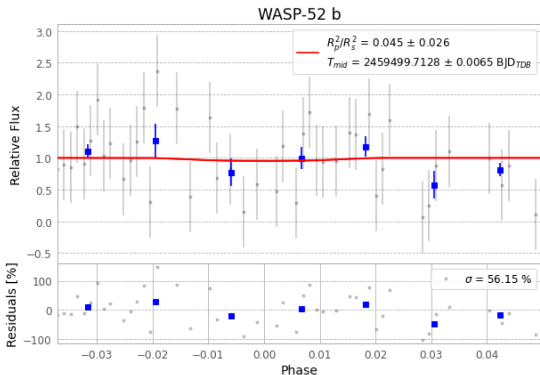
Figure 1 — FinalLightCurve_WASP-52 b_2021-10-11.png (SHA-256 5844a8818e77926a...)
