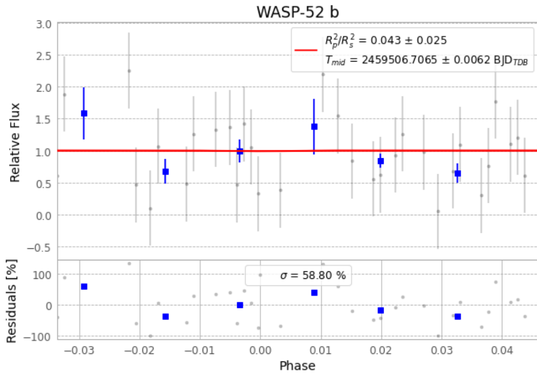
Figure 1 — FinalLightCurve_WASP-52 b_2021-10-18.png (SHA-256 a45017ff0a9e4a3d...)
