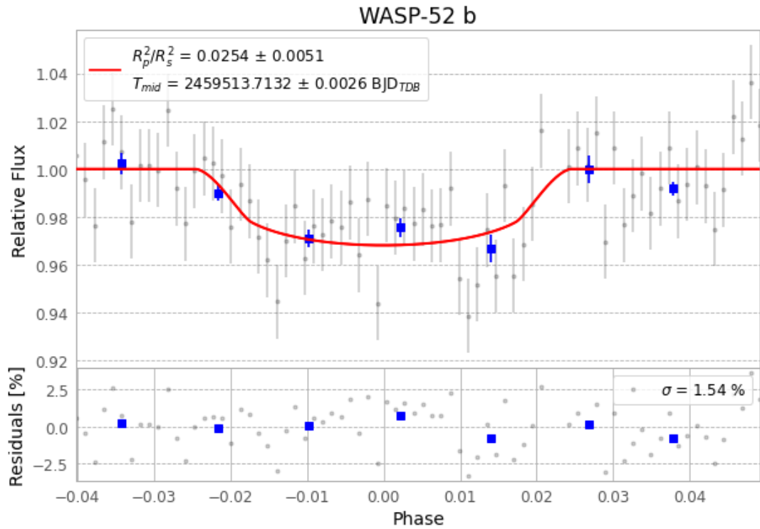
Figure 1 — FinalLightCurve_WASP-52 b_2021-10-25.png (SHA-256 1d41fd03d30d442b...)
