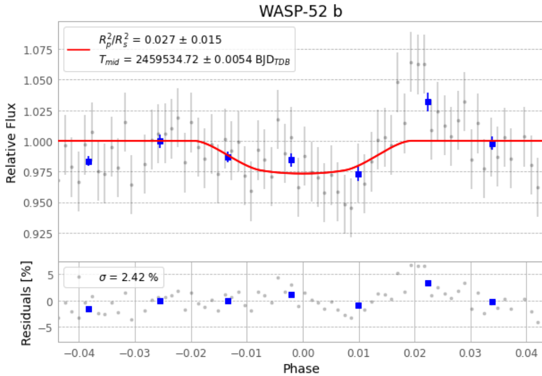
Figure 1 — FinalLightCurve_WASP-52 b_2021-11-15.png (SHA-256 e955fe66e3d9f108...)
