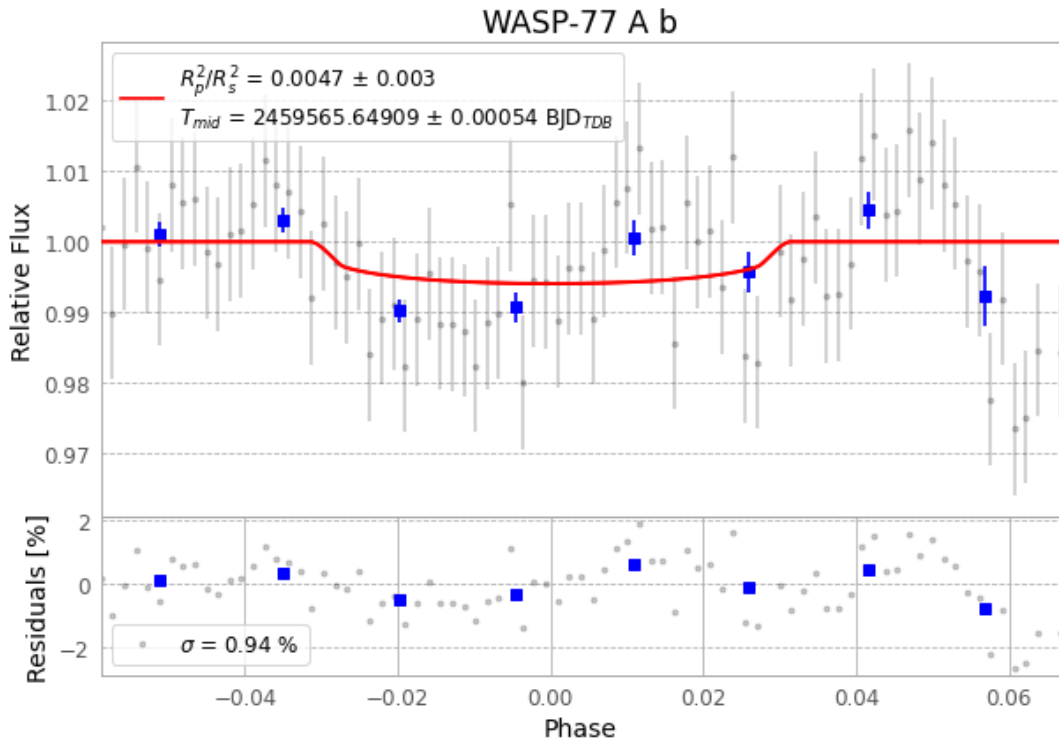
Figure 1 — FinalLightCurve_WASP-77 A b_2021-12-16.png (SHA-256 2f6daa265016cad1...)
