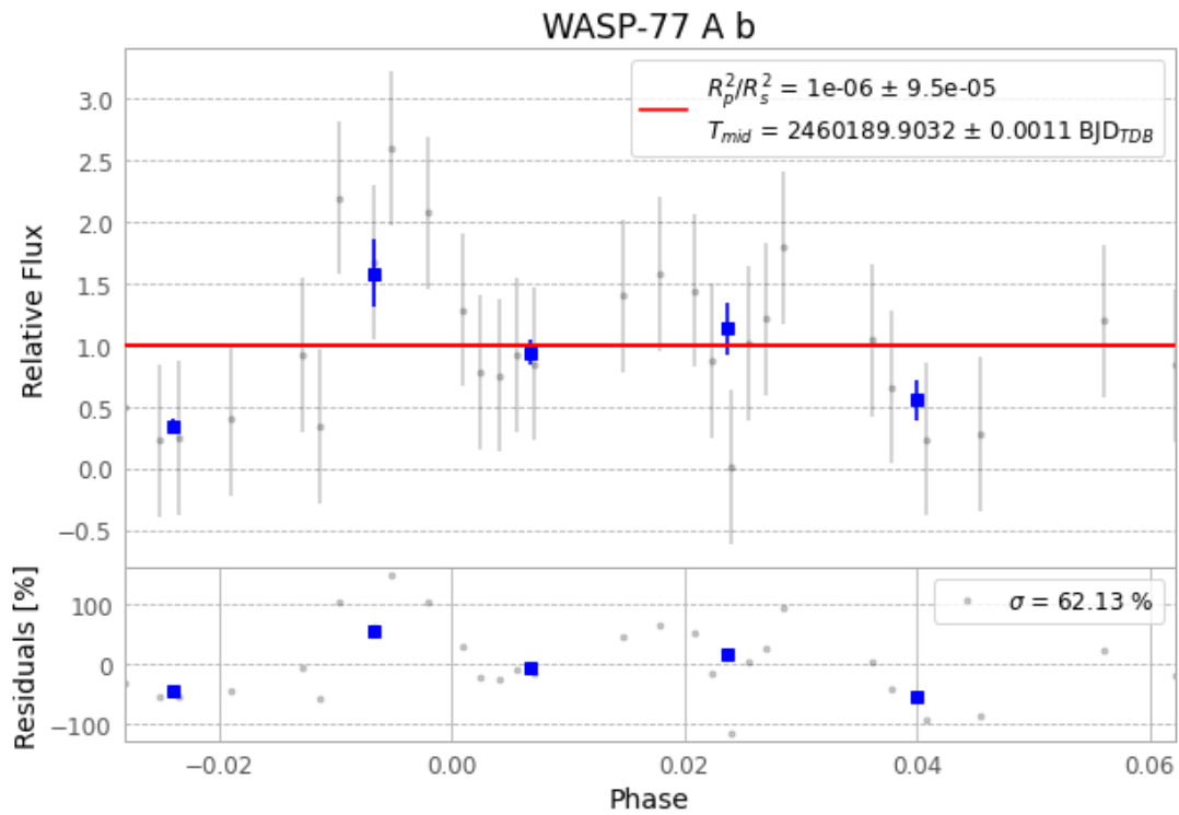
Figure 1 — FinalLightCurve_WASP-77 A b_2023-09-02.png (SHA-256 f742caa626754988...)
