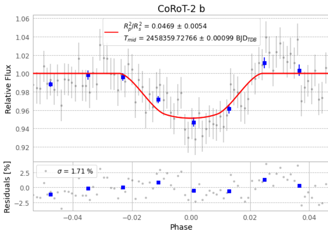
Figure 1 — FinalLightCurve_CoRoT-2 b_2018-08-28.png (SHA-256 6b8184539a6eba7b...)
