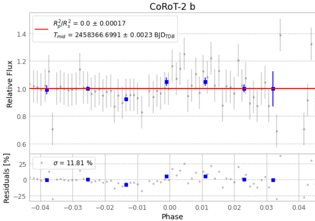
Figure 1 — FinalLightCurve_CoRoT-2 b_2018-09-04.png (SHA-256 acf6cb31bddefa94...)
