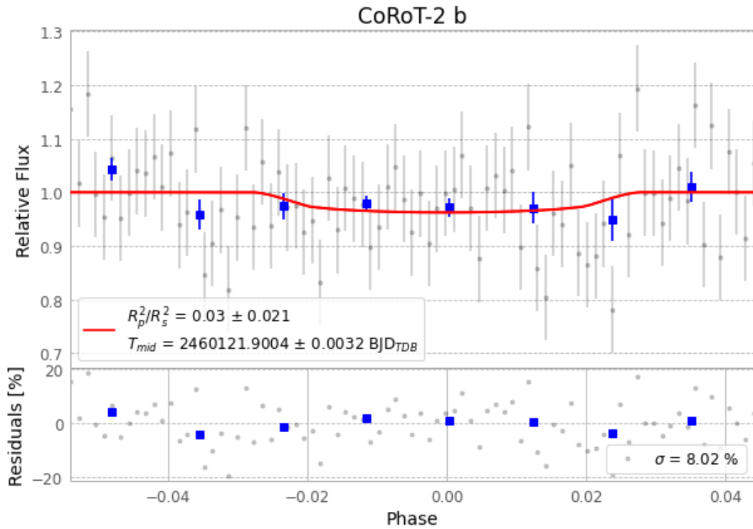
Figure 1 — FinalLightCurve_CoRoT-2 b_2023-06-26.png (SHA-256 ebd4225d7ee41b3b...)
