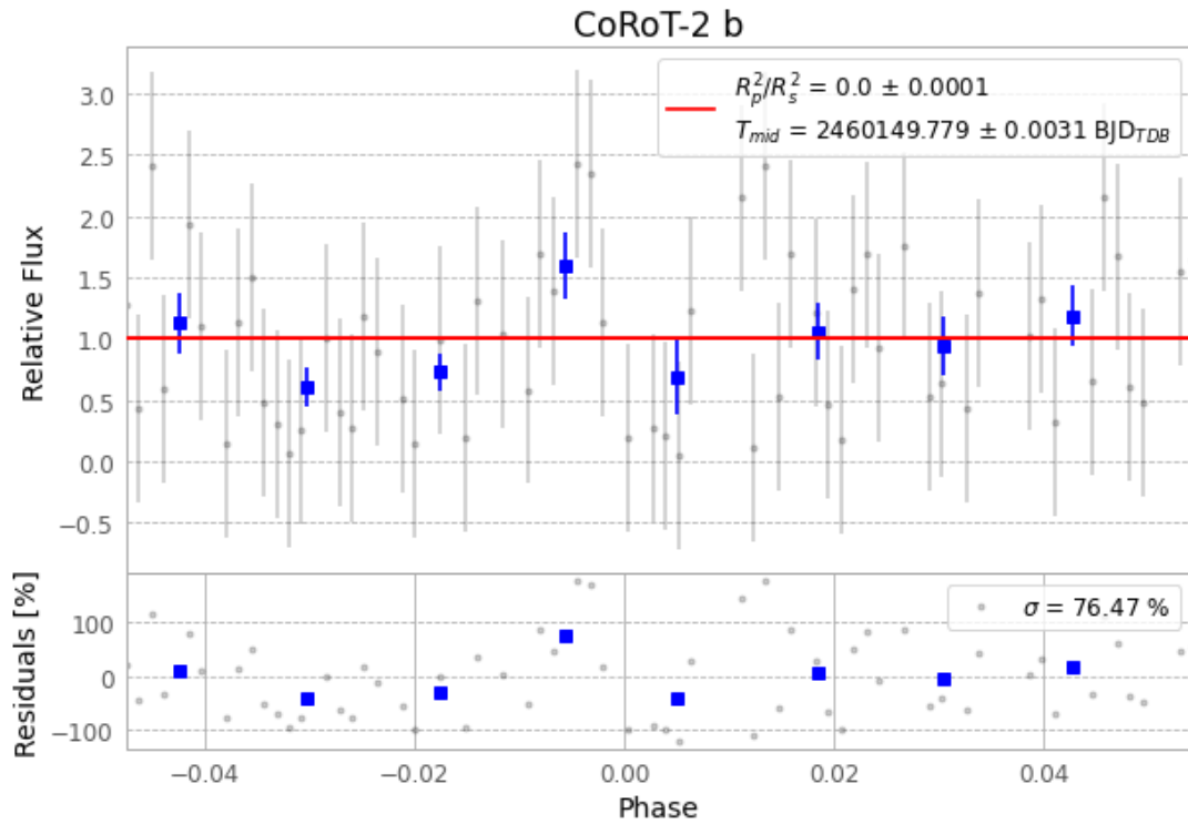
Figure 1 — FinalLightCurve_CoRoT-2 b_2023-07-23.png (SHA-256 ac48717a09a2b7a6...)
