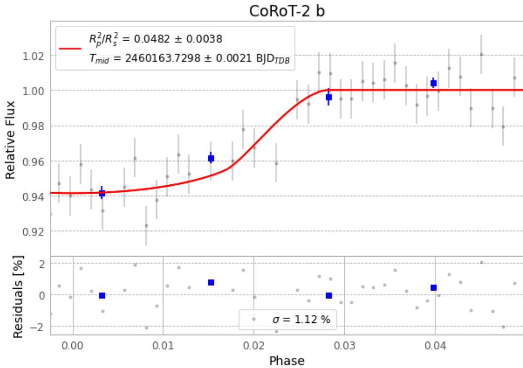
Figure 1 — FinalLightCurve_CoRoT-2 b_2023-08-06.png (SHA-256 dd30ae32e05b3e66...)
