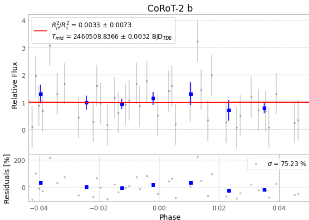
Figure 1 — FinalLightCurve_CoRoT-2 b_2024-07-16.png (SHA-256 c16165450e1e504d...)
