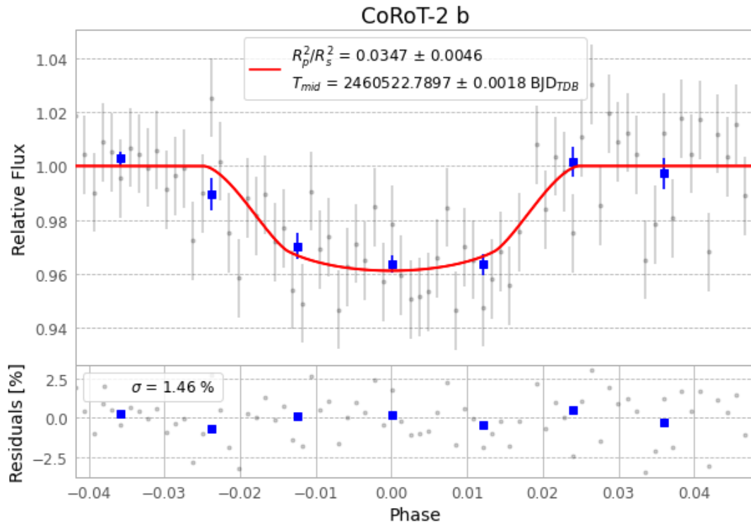
Figure 1 — FinalLightCurve_CoRoT-2 b_2024-07-30.png (SHA-256 f45b5ae0187fcaab...)
