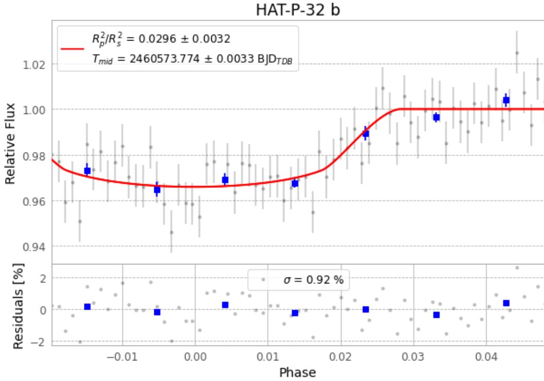
Figure 1 — FinalLightCurve_HAT-P-32 b_2024-09-19.png (SHA-256 be17a070f90a3454...)
