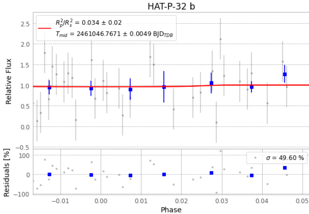
Figure 1 — FinalLightCurve_HAT-P-32 b_2026-01-05.png (SHA-256 decb3961b92c2e96...)
