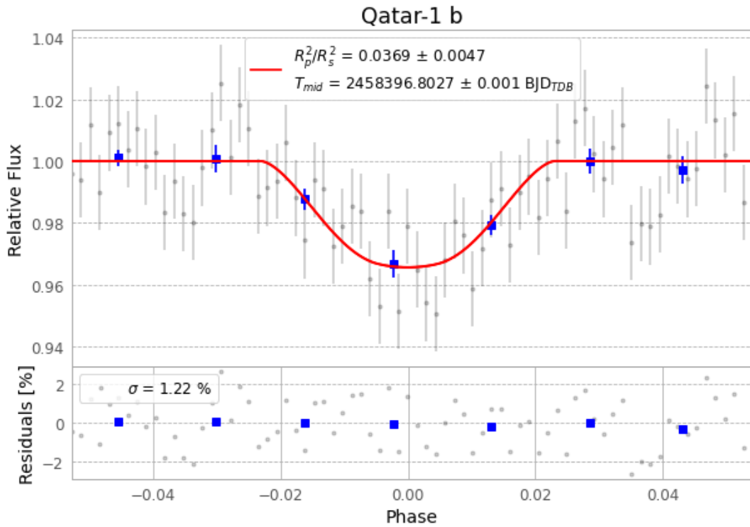
Figure 1 — FinalLightCurve_Qatar-1 b_2018-10-04.png (SHA-256 daf3a543dd2810cb...)
