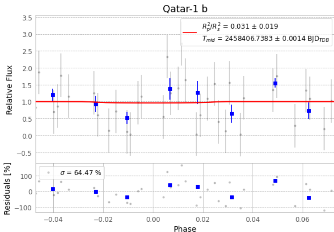
Figure 1 — FinalLightCurve_Qatar-1 b_2018-10-14.png (SHA-256 14cf54bf54aa9c29...)
