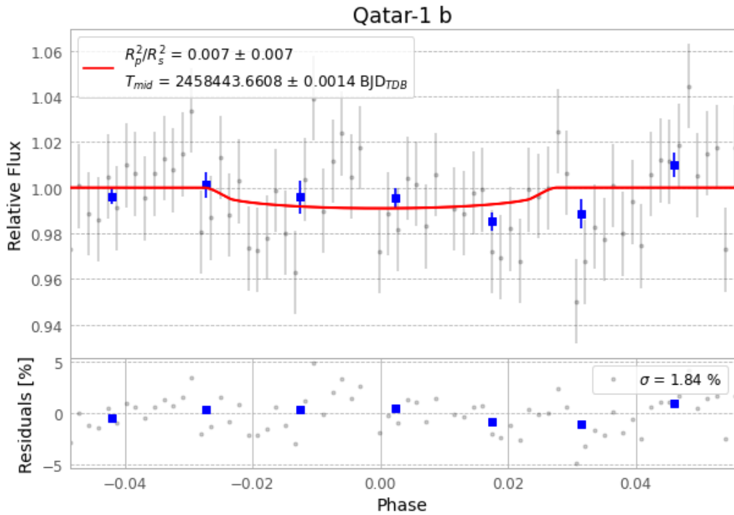
Figure 1 — FinalLightCurve_Qatar-1 b_2018-11-20.png (SHA-256 98d8f5174cdbd9d0...)
