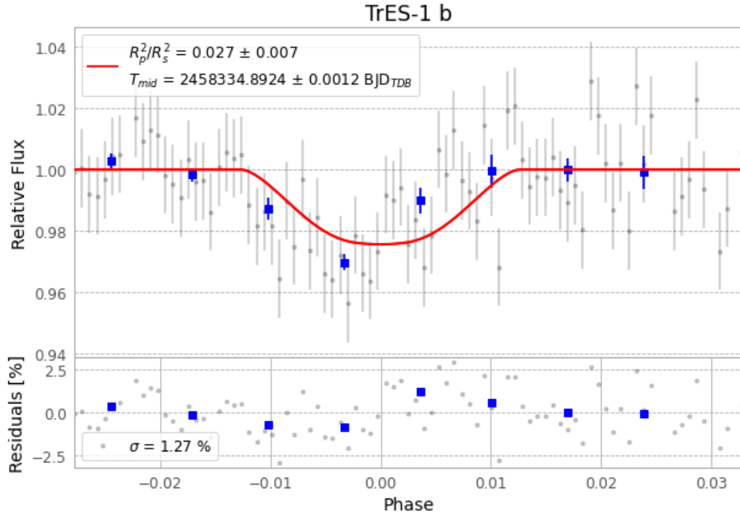
Figure 1 — FinalLightCurve_TrES-1 b_2018-08-04.png (SHA-256 307f7411ebf430e6...)
