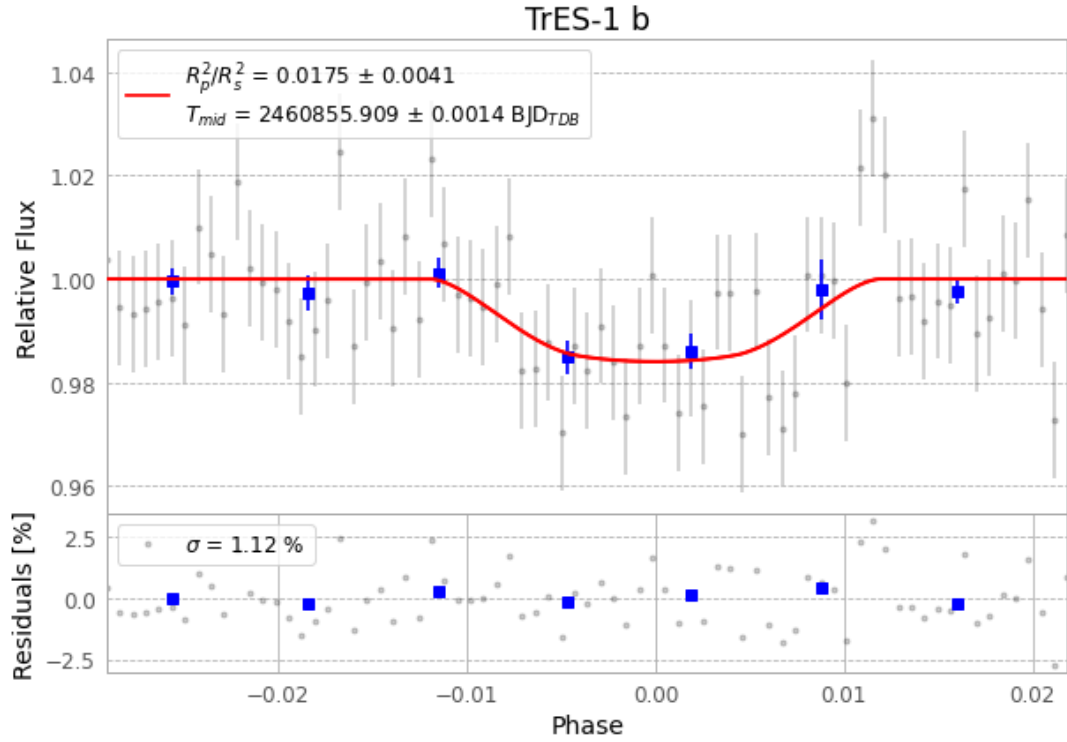
Figure 1 — FinalLightCurve_TrES-1 b_2025-06-29.png (SHA-256 27b070192ae60d21...)
