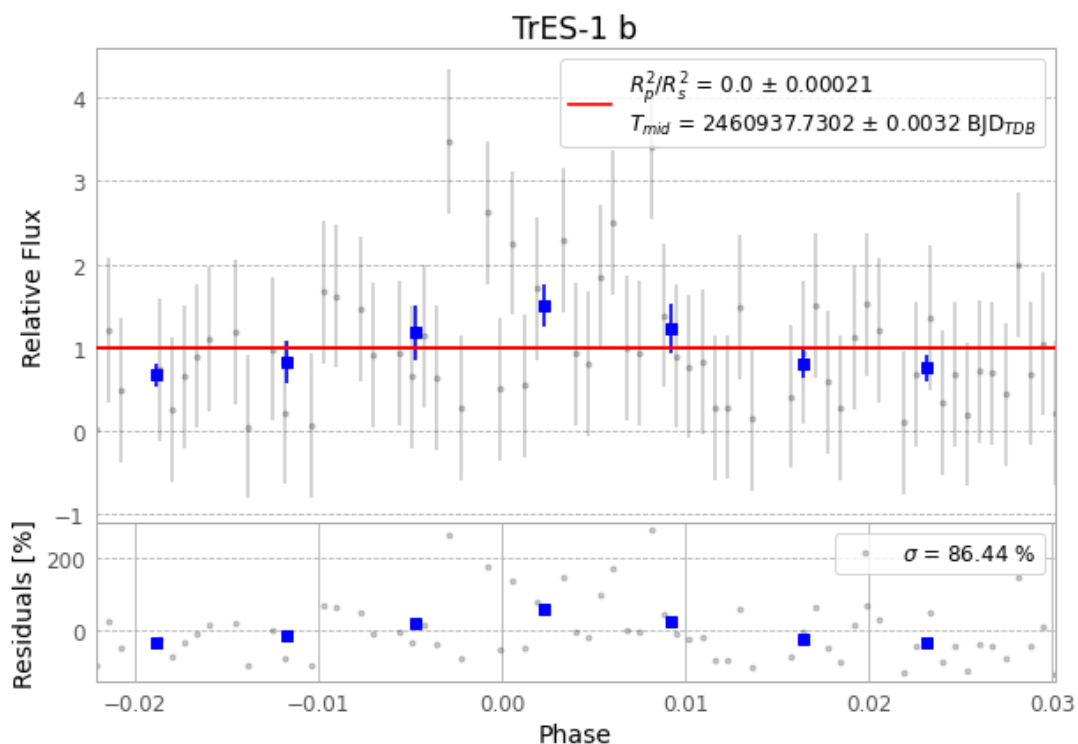
Figure 1 — FinalLightCurve_TrES-1 b_2025-09-18.png (SHA-256 8292471c0953ce64...)
