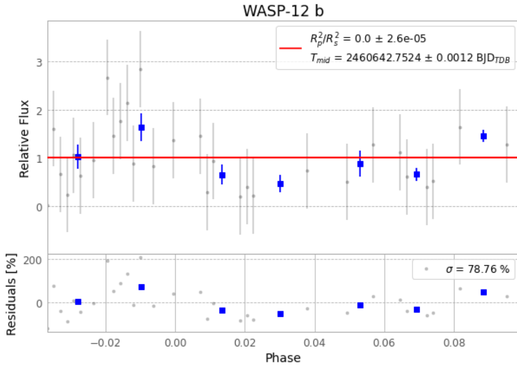
Figure 1 — FinalLightCurve_WASP-12 b_2024-11-27.png (SHA-256 bc128f9a3d0a5df9...)
