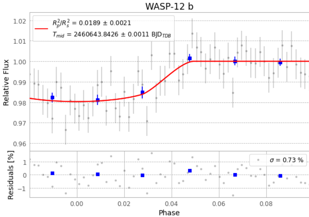
Figure 1 — FinalLightCurve_WASP-12 b_2024-11-29.png (SHA-256 dbd8b46259081bf7...)
