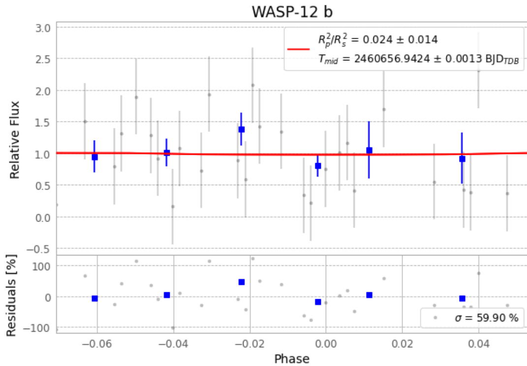
Figure 1 — FinalLightCurve_WASP-12 b_2024-12-12.png (SHA-256 67fd21e7306f438b...)
