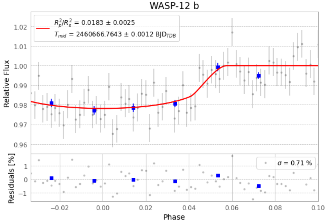
Figure 1 — FinalLightCurve_WASP-12 b_2024-12-21.png (SHA-256 57164c41eb69288b...)
